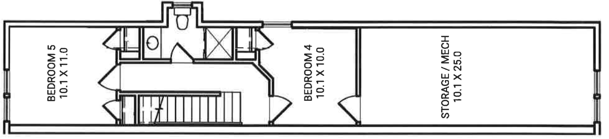
Attic
