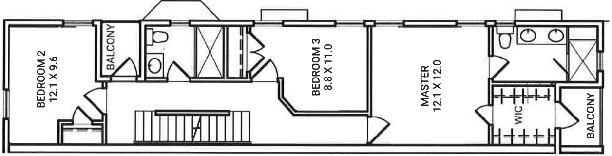
Second Floor
